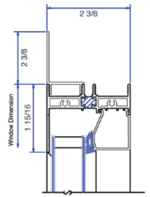
HEAD AT FIXED W/ FLUSH FLANGE
