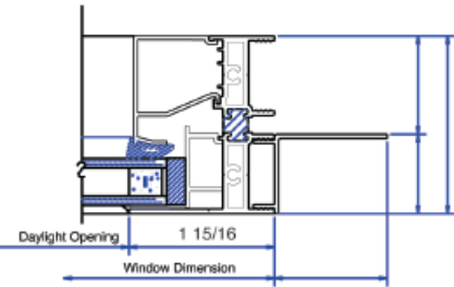
JAMB AT FIXED W/ 5/8" GLAZING
