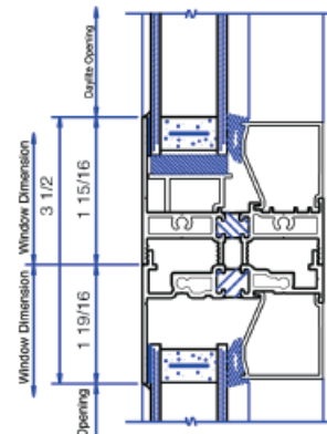
STACKING HEAD
