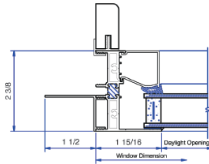
JAMB AT FIXED W/ OPTIONAL NAILING FLANGE & OPTIONAL EXTENSION JAMB
