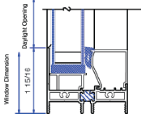
SILL AT FIXED
